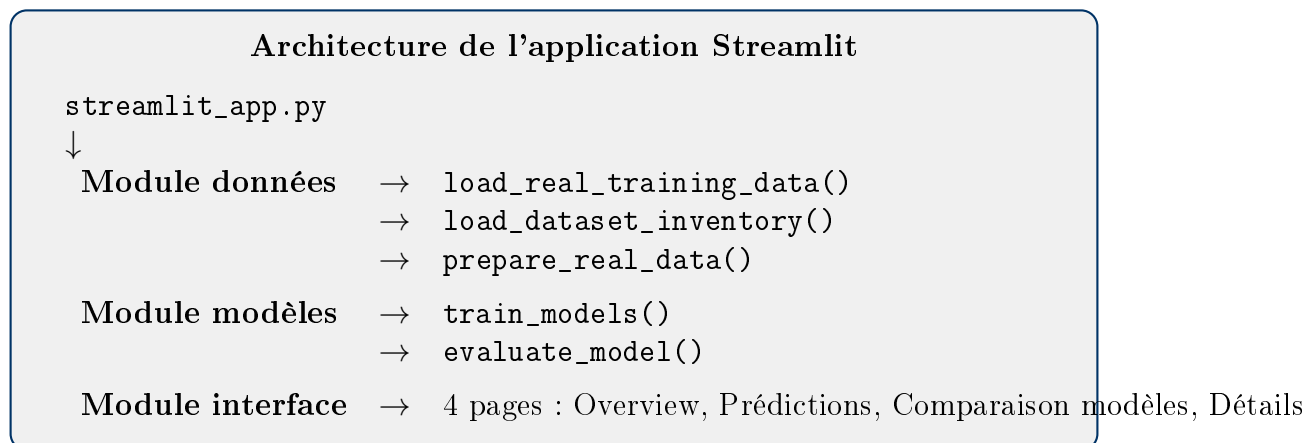
FIGURE 14 – Architecture modulaire de l'application Streamlit
