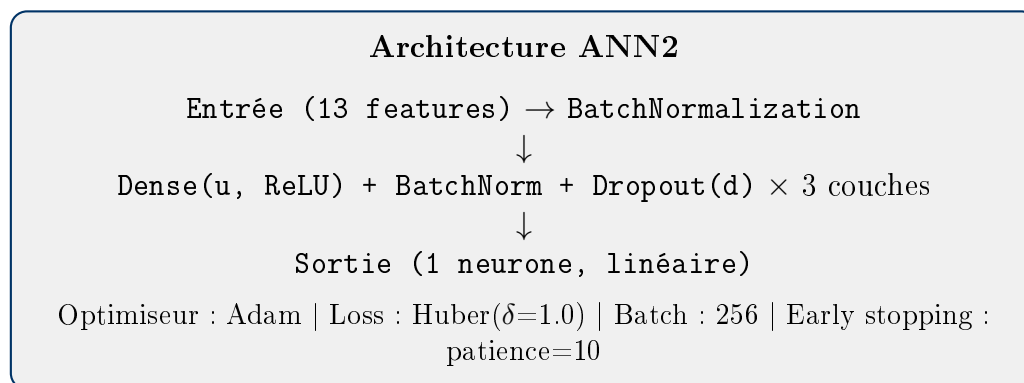
FIGURE 12 – Architecture Deep + BatchNorm (ANN2)
